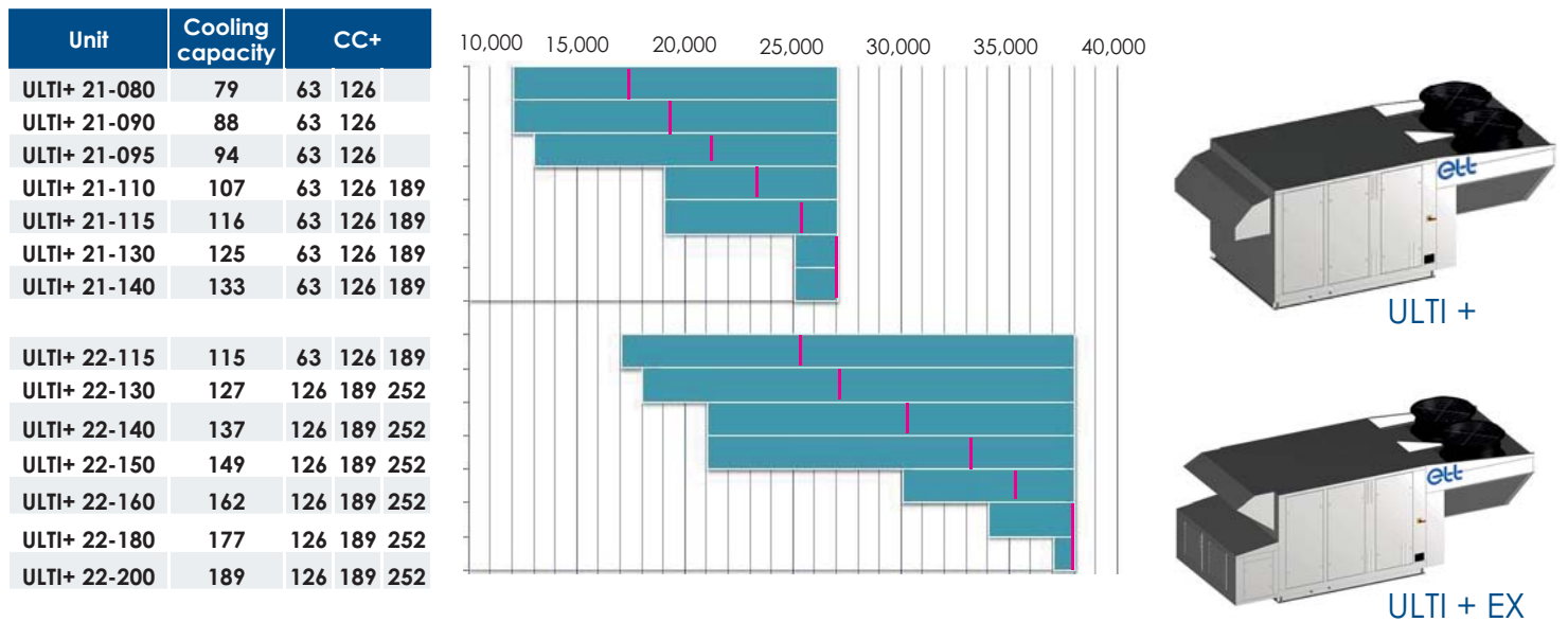
Flow rates (m 3 /h) & rated air flow rate (l)
